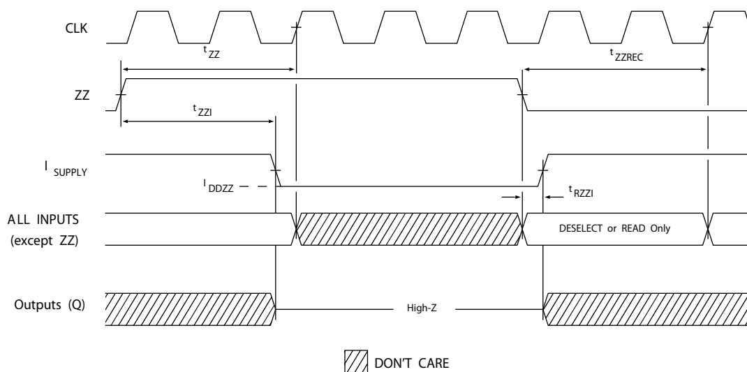
Figure 8. ZZ Mode Timing
