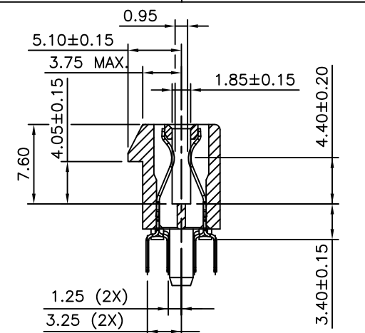
SECTION P-P
