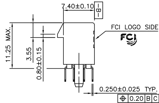
SECTION P-P
