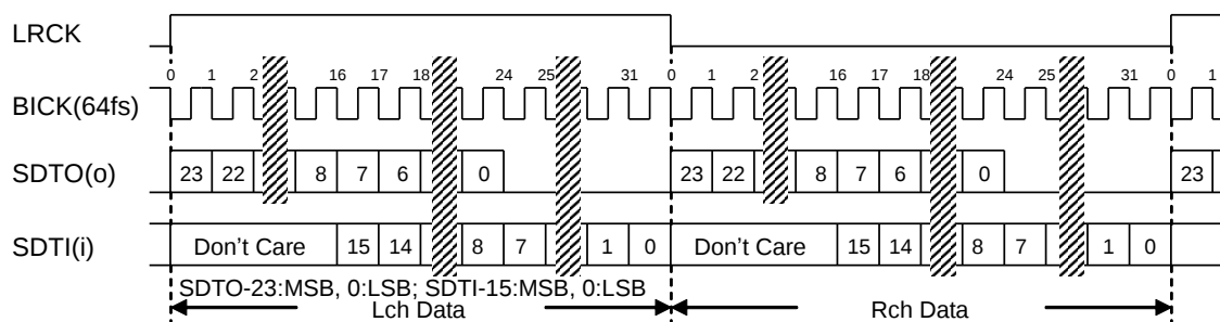
Figure 17. Mode 0/8 Timing
