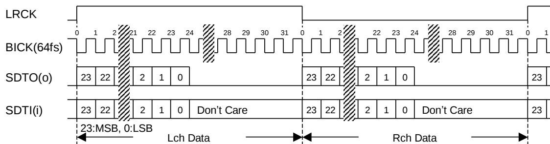
Figure 19. Mode 2/10 Timing
