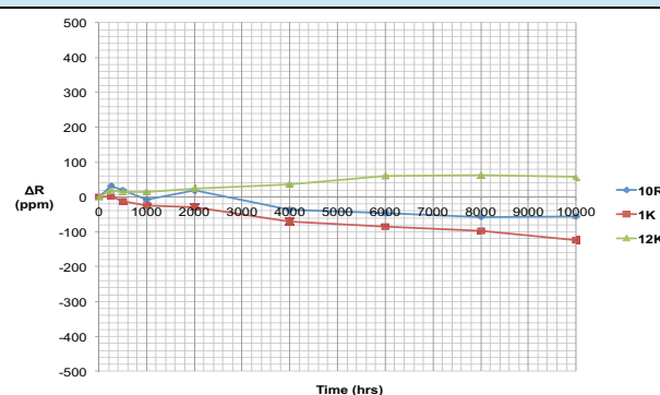
FIGURE 6 - LOAD LIFE TEST FOR 10,000 HRS @0.3W, +70°C; VSMP 1206, N=40
