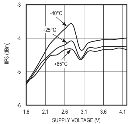
MAX2686L IN-BAND IIP3 vs. SUPPLY VOLTAGE AND TEMPERATURE (TWO TONES LOCATED AT 1MHz AND 2MHz OFFSET WITH -30dBm/TONE)
