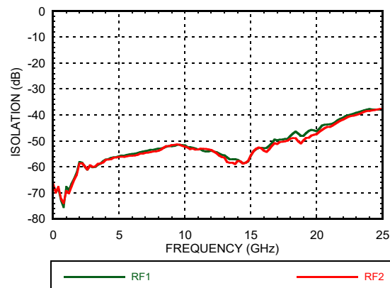
Isolation
