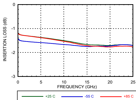
Insertion Loss
