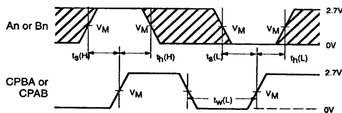
Waveform 4. Data Setup and Hold Times
