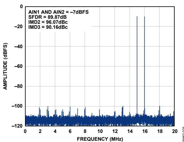
Figure 25. Two-Tone 32k FFT with f_{\text{IN1}} = 15 MHz and f_{\text{IN2}} = 16 MHz, AD9222-40
