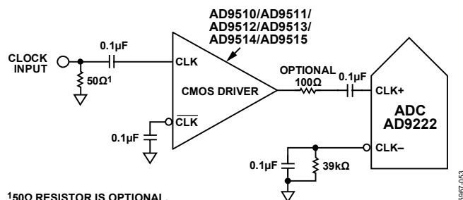
Figure 48. Single-Ended 1.8 V CMOS Sample Clock
