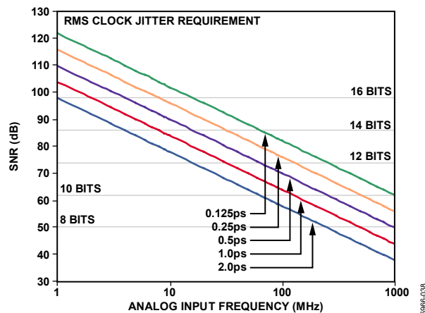
Figure 50. Ideal SNR vs. Input Frequency and Jitter
