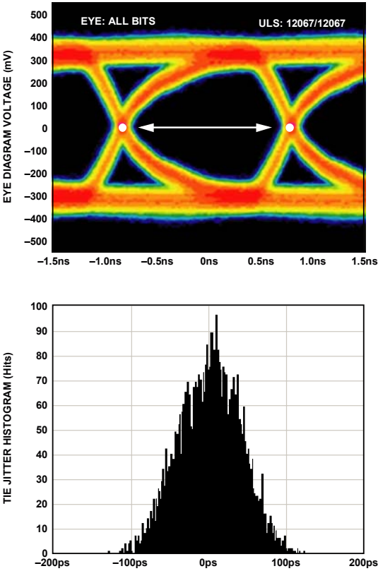
Figure 54. Data Eye for LVDS Outputs in ANSI Mode with Trace Lengths Greater than 24 Inches on Standard FR-4, AD9222-50
