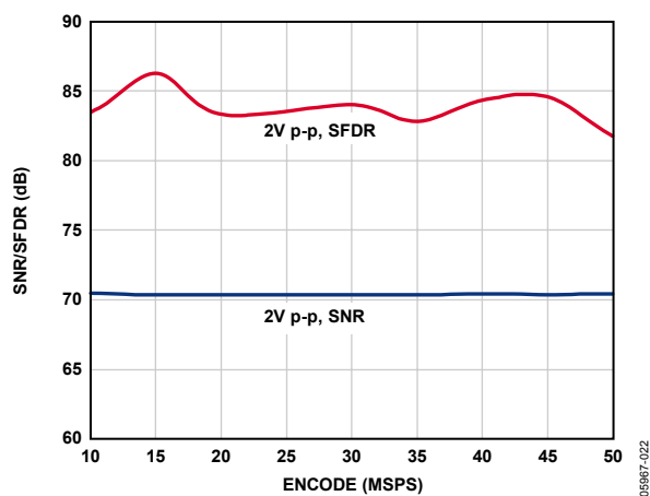
Figure 22. SNR/SFDR vs. f_{\text{SAMPLE}} , f_{\text{IN}} = 20.1 MHz, AD9222-50
