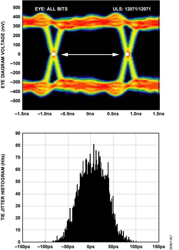
Figure 53. Data Eye for LVDS Outputs in ANSI Mode with Trace Lengths Less than 24 Inches on Standard FR-4, AD9222-50
