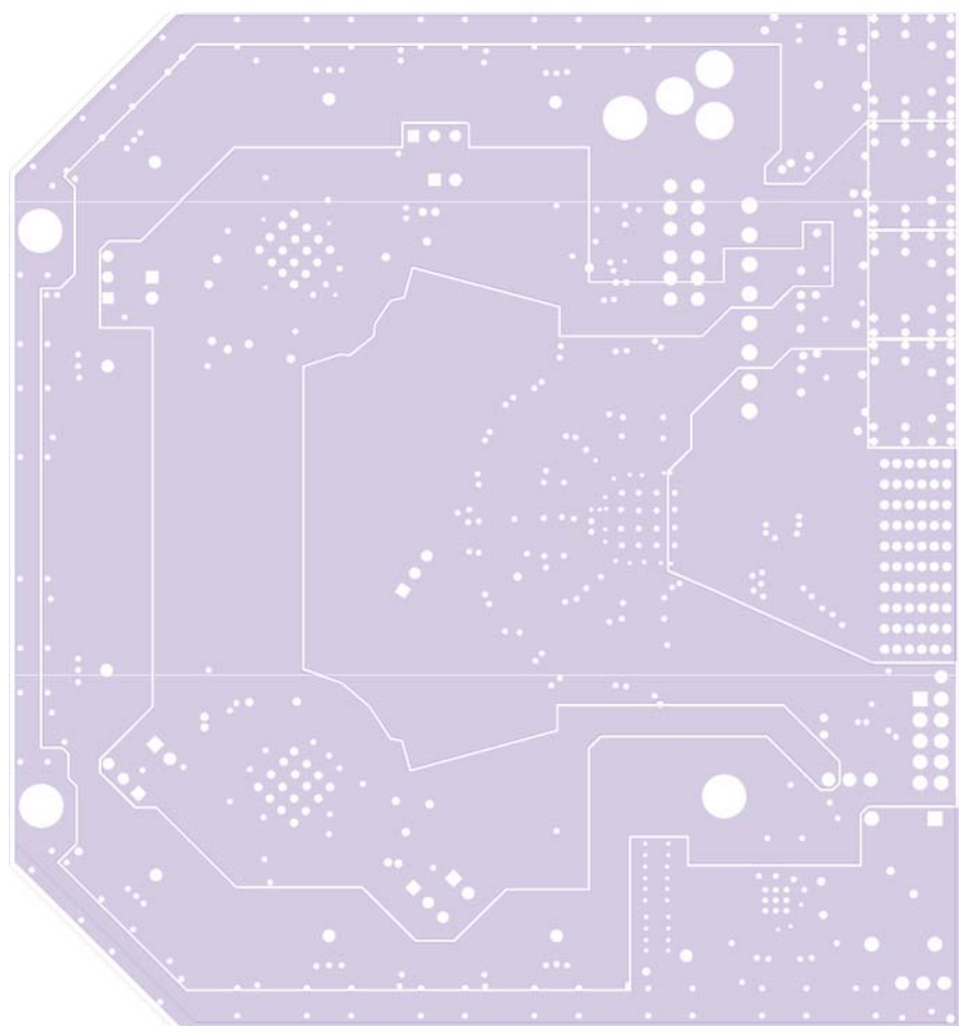
Figure 76. Evaluation Board Layout, Power Plane
