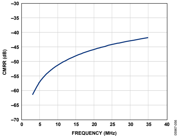
Figure 34. CMRR vs. Frequency, AD9222-50
