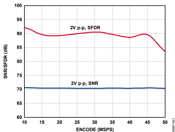
Figure 21. SNR/SFDR vs. f_{\text{SAMPLE}} , f_{\text{IN}} = 2.61 MHz, AD9222-50
