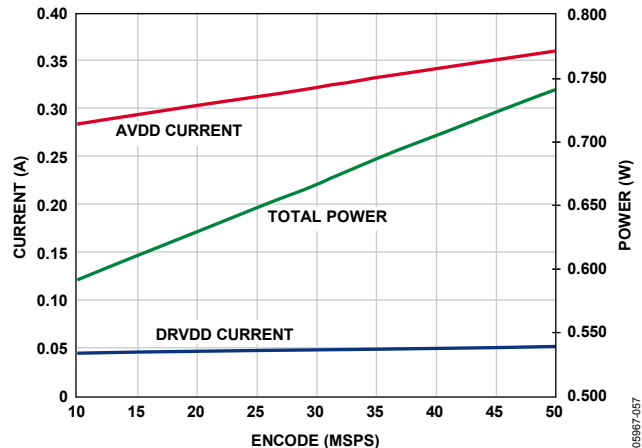
Figure 51. Supply Current vs. f_{\text{SAMPLE}} for f_{\text{IN}} = 10.3 \text{ MHz} , AD9222-50
