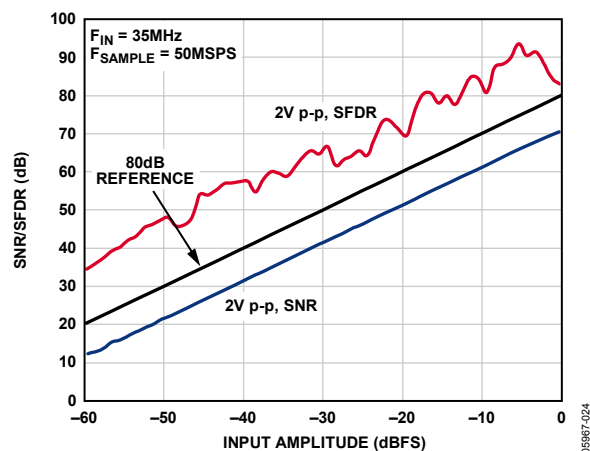
Figure 24. SNR/SFDR vs. Analog Input Level, f_{\text{IN}} = 35 MHz, AD9222-50
