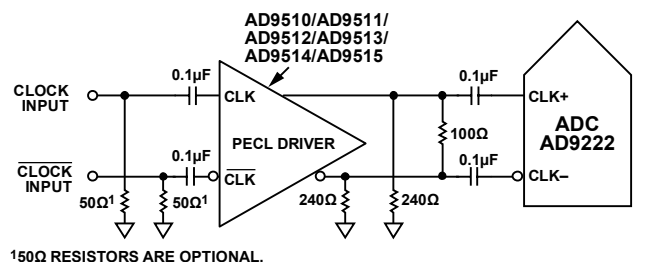
Figure 46. Differential PECL Sample Clock
