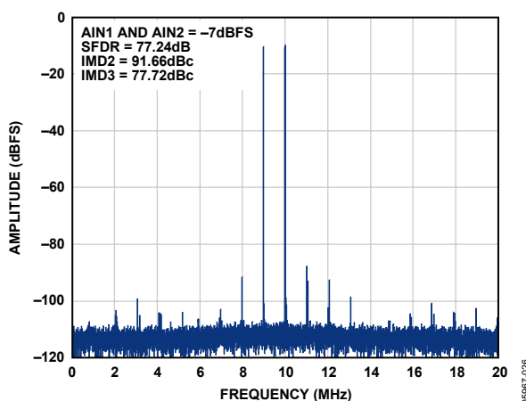
Figure 26. Two-Tone 32k FFT with f_{\text{IN1}} = 70 MHz and f_{\text{IN2}} = 71 MHz, AD9222-40
