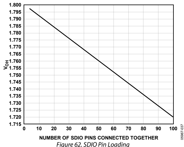
Figure 62. SDIO Pin Loading
