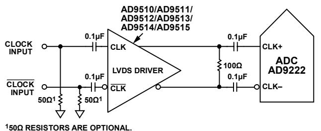
Figure 47. Differential LVDS Sample Clock
