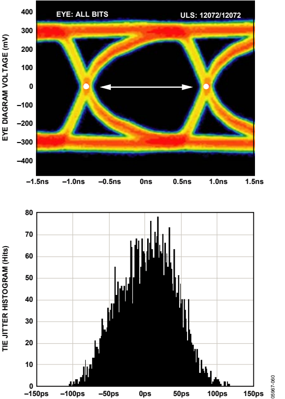
Figure 55. Data Eye for LVDS Outputs in ANSI Mode with 100 \Omega Termination on and Trace Lengths Greater than 24 Inches on Standard FR-4, AD9222-50
