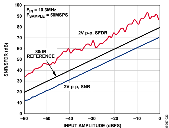
Figure 23. SNR/SFDR vs. Analog Input Level, f_{\text{IN}} = 10.3 MHz, AD9222-50
