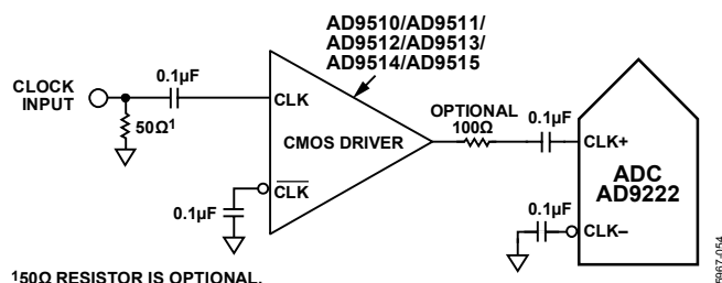
Figure 49. Single-Ended 3.3 V CMOS Sample Clock
