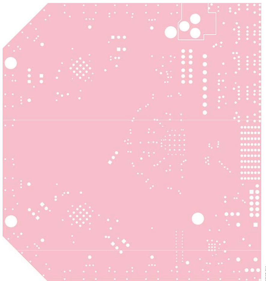
Figure 75. Evaluation Board Layout, Ground Plane
