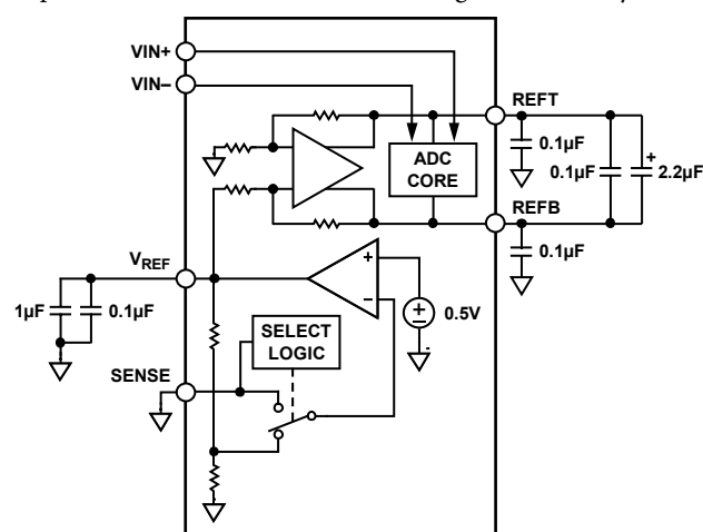
Figure 58. Internal Reference Configuration
