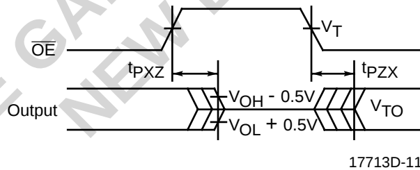
e. \overline{\text{OE}} to output disable/enable
