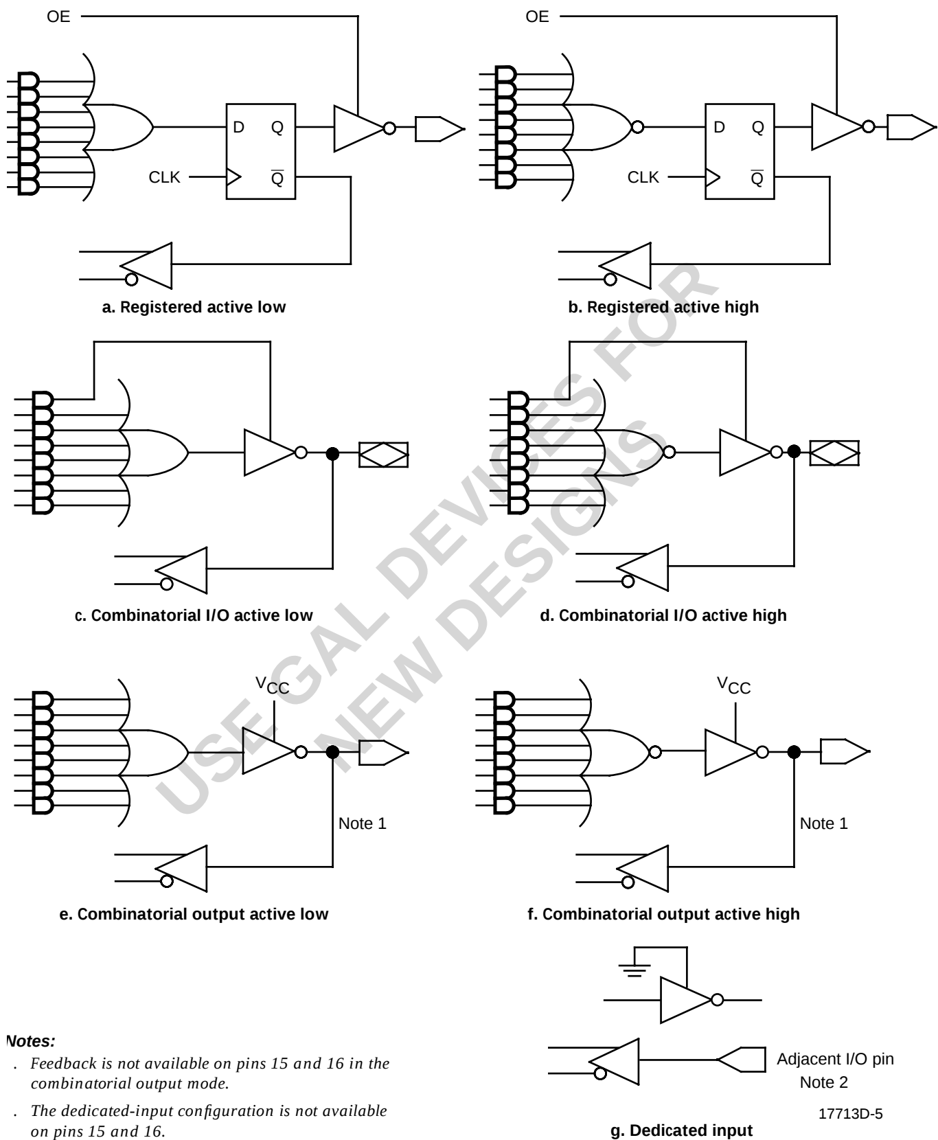
Figure 2. Macrocell Configurations
