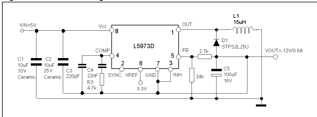
Figure 17. Buck-boost regulator
