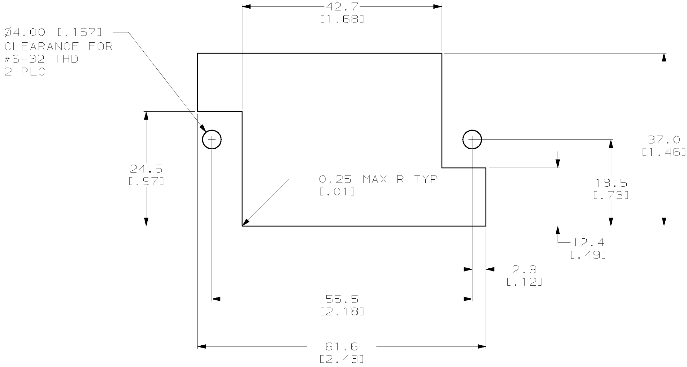
RECOMMENDED STATIONARY MOUNT PANEL CUTOUT #6 EXTERNAL VIEW
