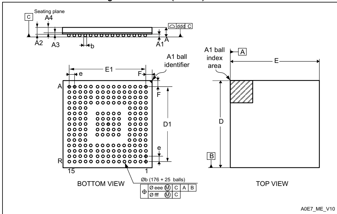
Figure 91. UFBGA(176+25) - Outline
