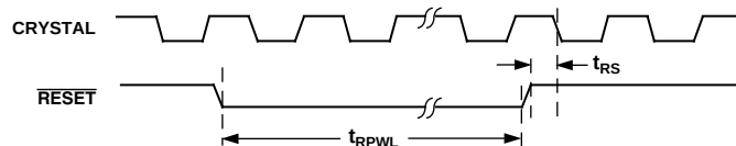
Figure 27. Reset Timing
