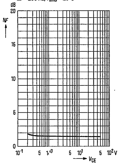
Noise figure NF = f(V_{CE}) I_G = 0.2 \text{ mA}; R_G = 2 \text{ k}\Omega; f = 1 \text{ kHz} \Delta f = 200 \text{ Hz}; T_{amb} = 25^\circ\text{C}
