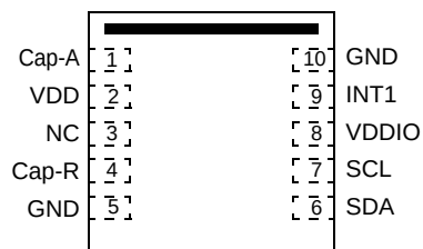
Pin Connections
