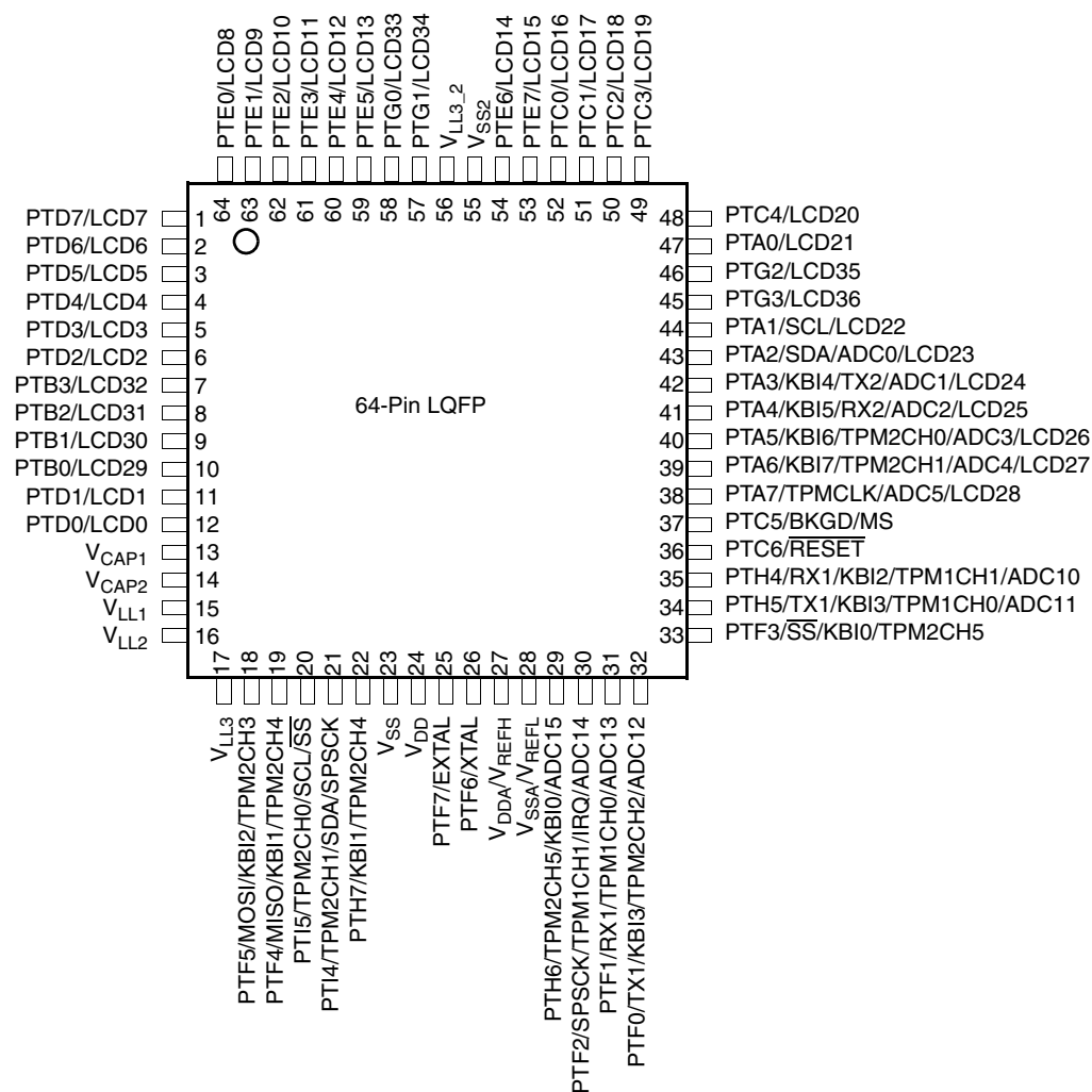
Figure 3. 64-Pin LQFP
