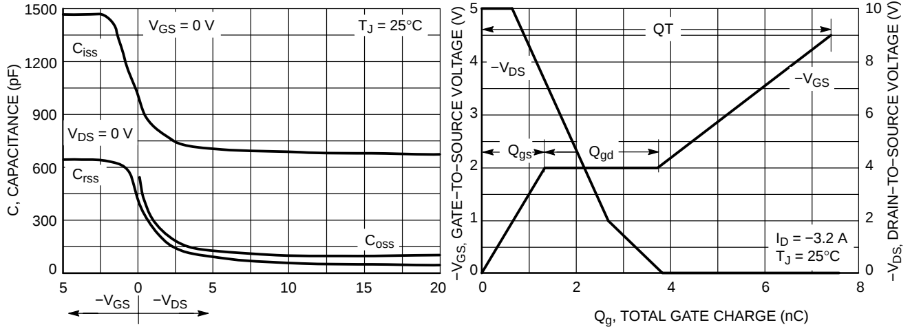
Figure 7. Capacitance Variation
