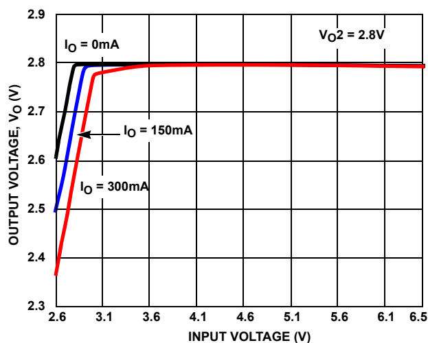
FIGURE 5. OUTPUT VOLTAGE vs INPUT VOLTAGE ( V_{O2} = 2.8\text{V} )
