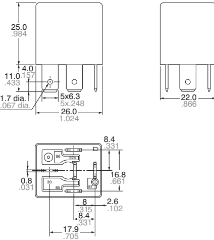
External dimensions
