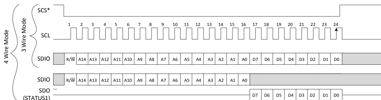
Figure 56. SPI Read
