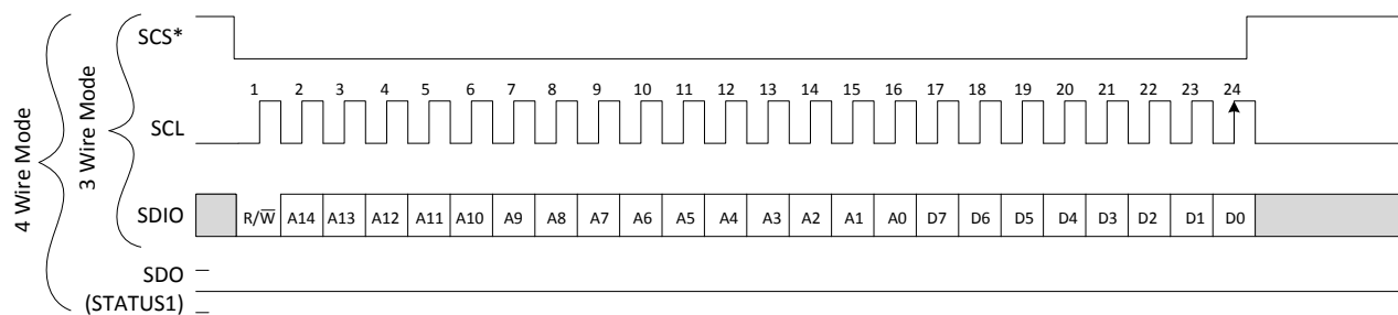
Figure 55. SPI Write
