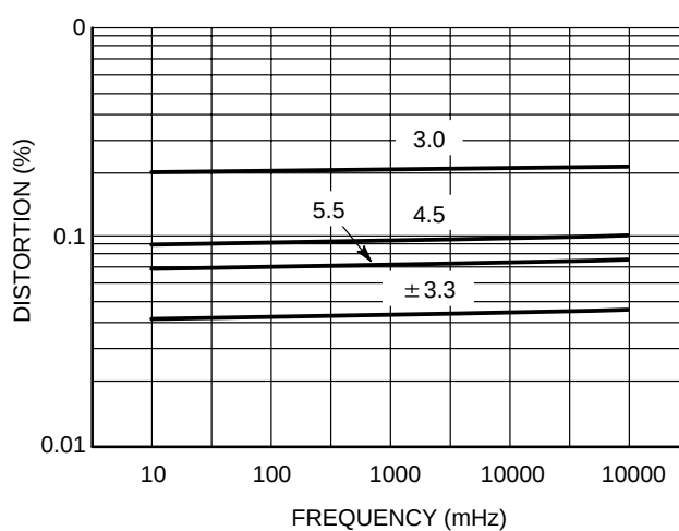
Figure 13. Total Harmonic Distortion
