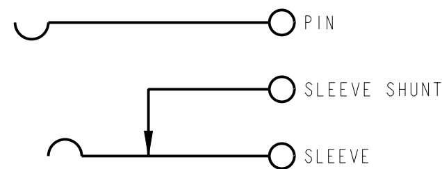
CIRCUIT DIAGRAM
