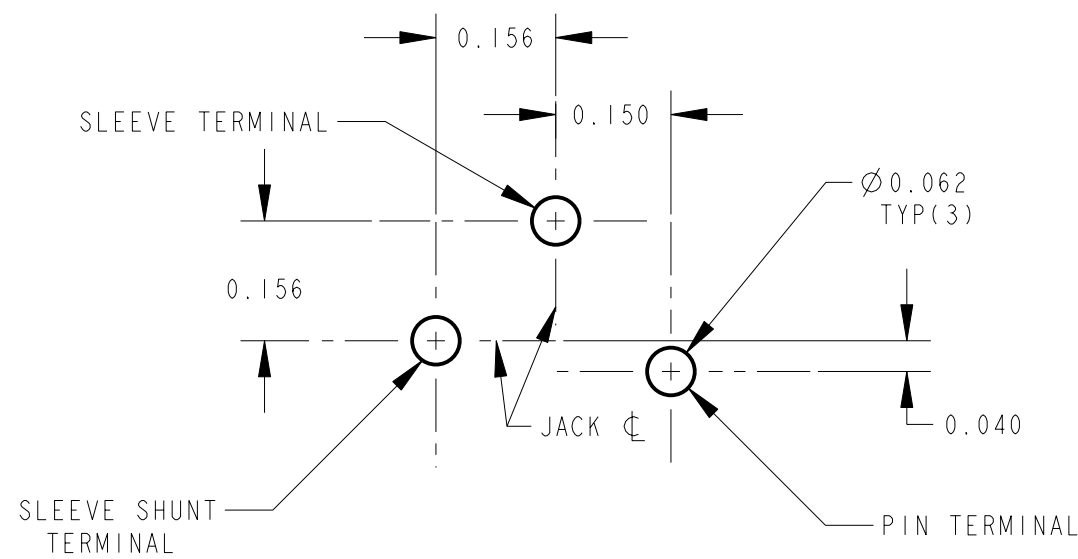
PC BOARD LAYOUT
