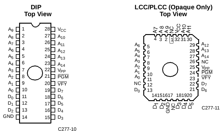
Figure 1. Programming Pinouts
