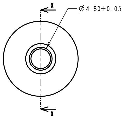
BOTTOM TOOL
