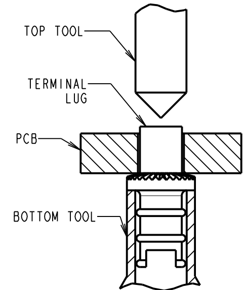
APPLICATION DIAGRAM
