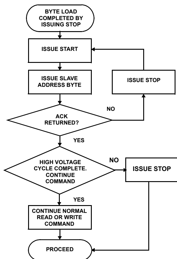
FIGURE 8. ACKNOWLEDGE POLLING SEQUENCE
