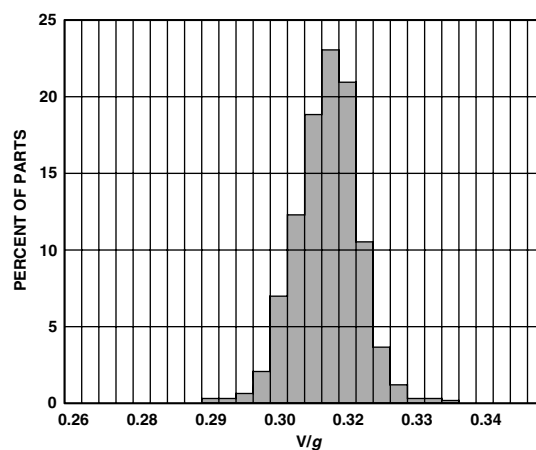
TPC 6. X-Axis Sensitivity Distribution at X_{FILT} , V_{DD} = 5\text{ V}
