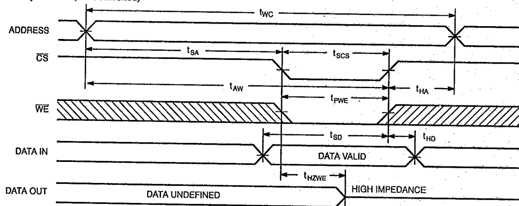
Write Cycle No. 2 ( \overline{CS} Controlled) [8,9]
