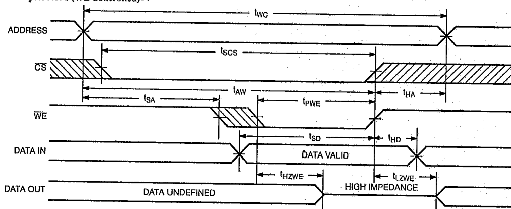
Write Cycle No. 1 ( \overline{WE} Controlled) [8]
