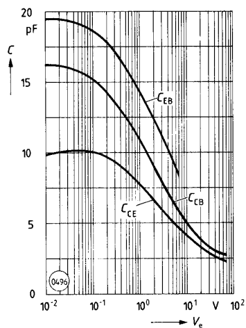
Figure 20. Transistor Capacitance C=f(V_O) ( T_A=25^\circ\text{C} , f=1.0\text{ MHz} )
