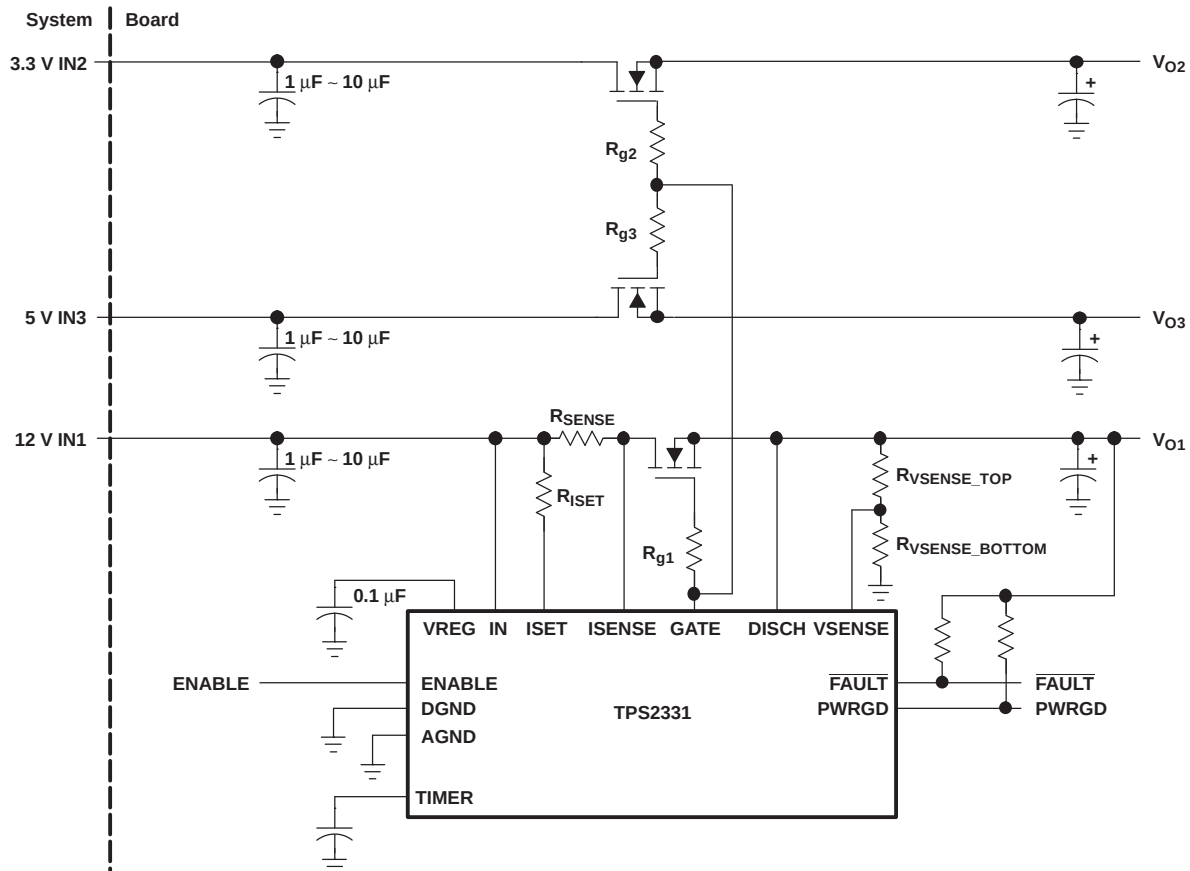
Figure 19. Three-Channel Application
