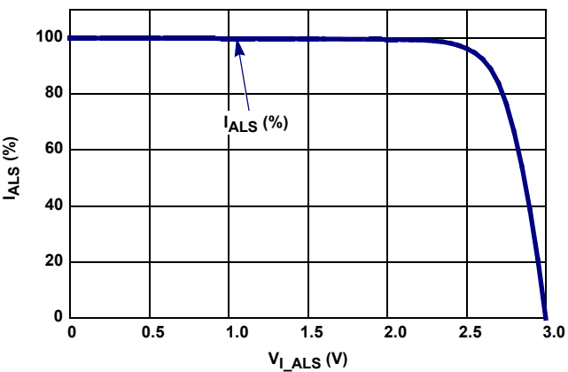
FIGURE 15. COMPLIANCE VOLTAGE ( V_{I\_ALS} ) EFFECTS ON I_{ALS} (REFERENCED TO V_{I\_ALS} = 0V )
