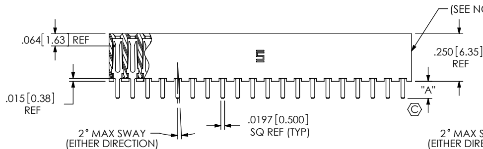
FIG 1 SQT-120-0T-XX-6 SHOWN
