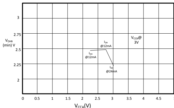
Figure 9-2. V_{OHB(min)} vs V_{CCA}
