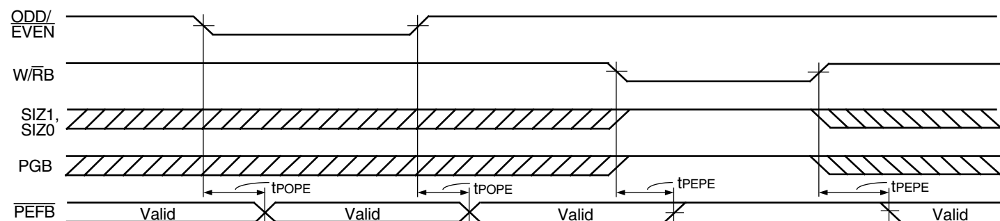
Figure 16. ODD/ \overline{EVEN} , \overline{W/RA} , MBA, and PGA to \overline{PEFA} Timing
