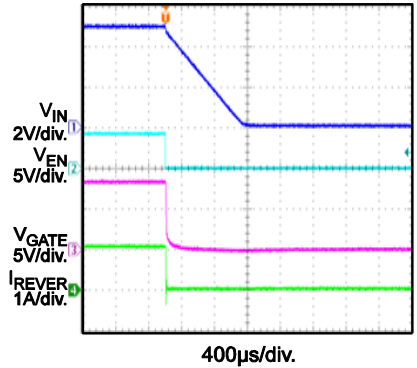
Reverse Current Protection during EN Shutdown V_{OUT} = 5V , Pull EN Low
