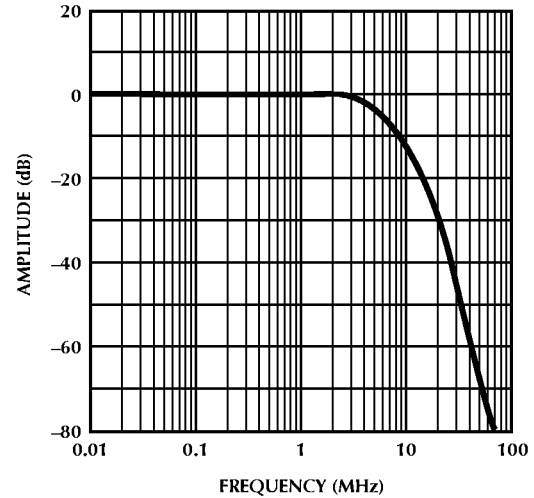
Figure 2. Passband/Stopband Rejection Ratios (Normalized) All outputs.
