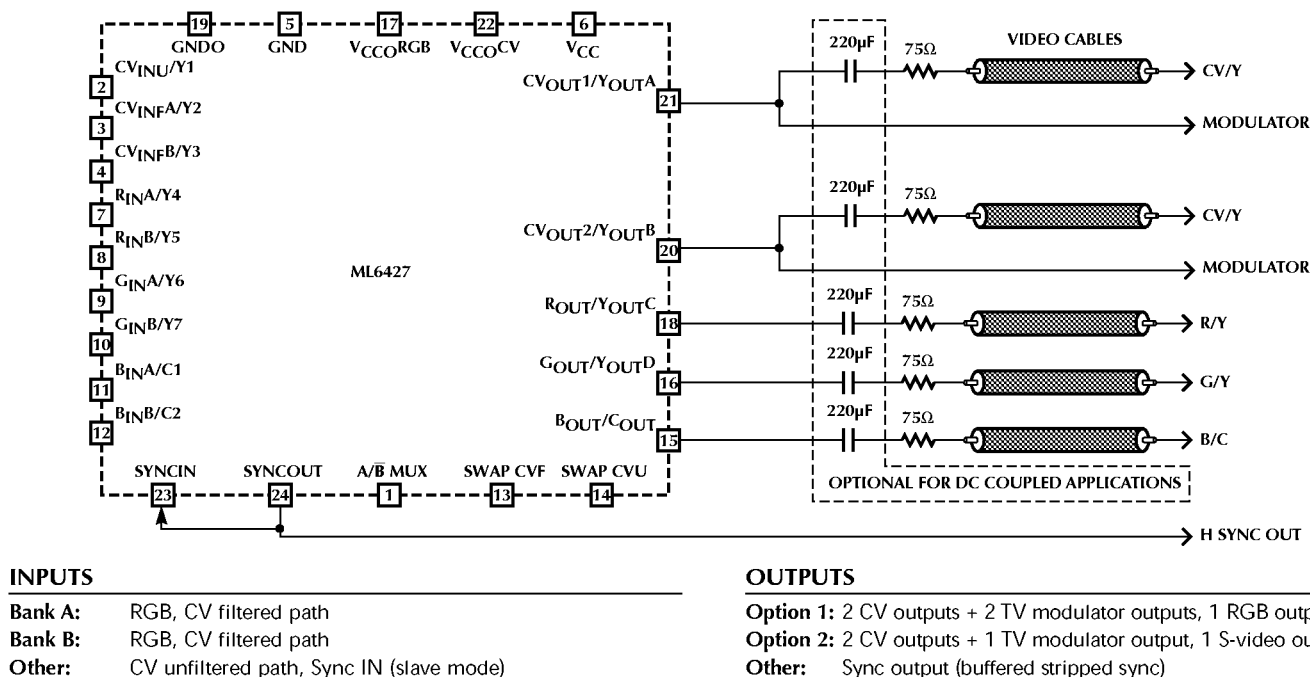
Figure 4. Basic Application for NTSC
