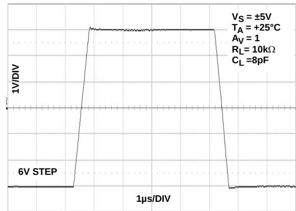
FIGURE 22. LARGE SIGNAL TRANSIENT RESPONSE
