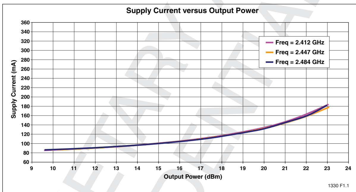
Figure 9: Supply Current versus Output Power
