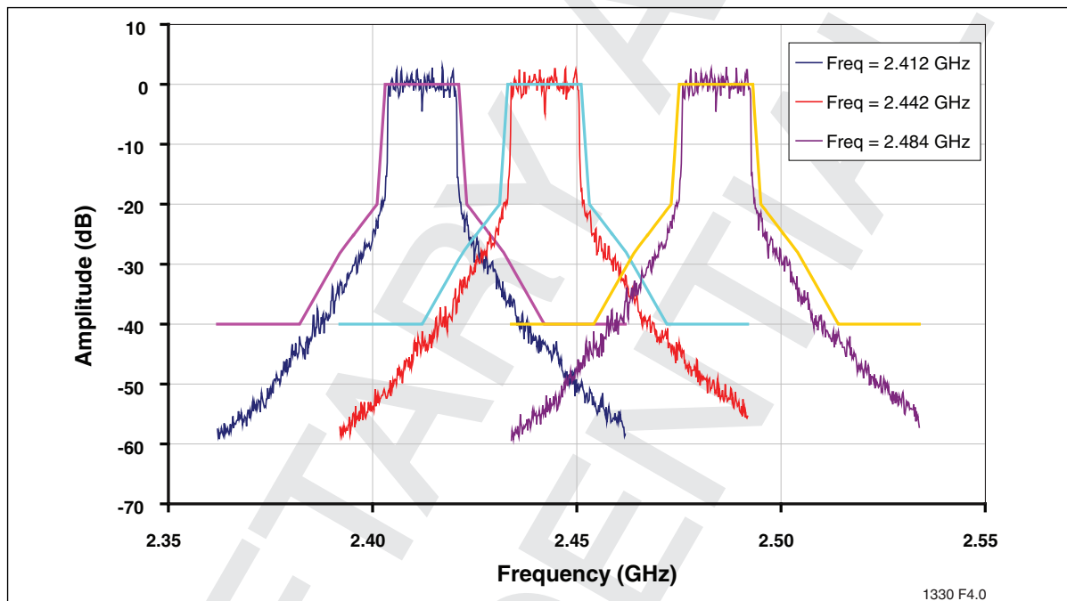
Figure 13: 802.11g Spectrum Mask at 23 dBm
