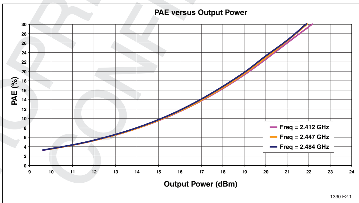
Figure 10: Power Added Efficiency (PAE) versus Output Power
