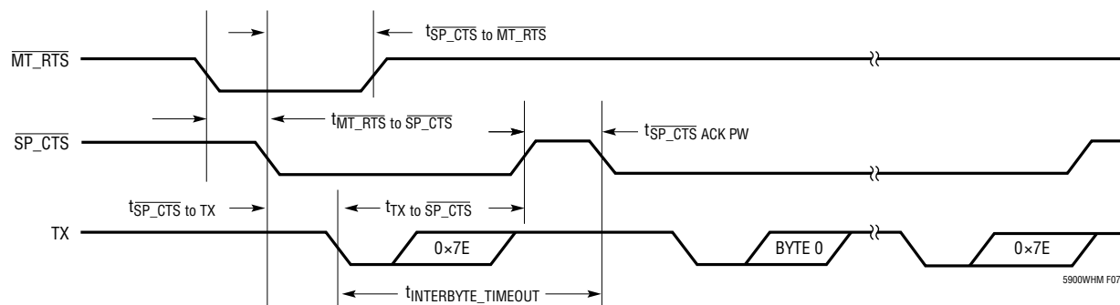
Figure 7. Flow Control Timing
