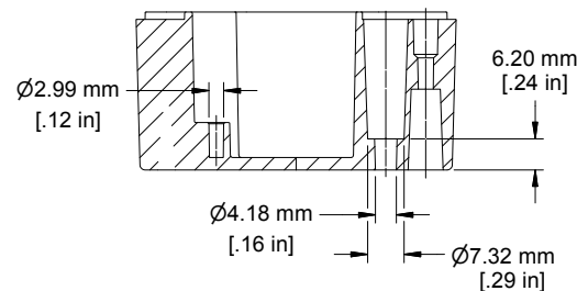
SECTION C-C Side View of Box
