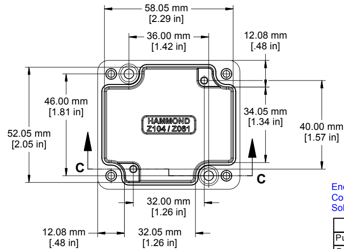
Top View Looking Inside Box
