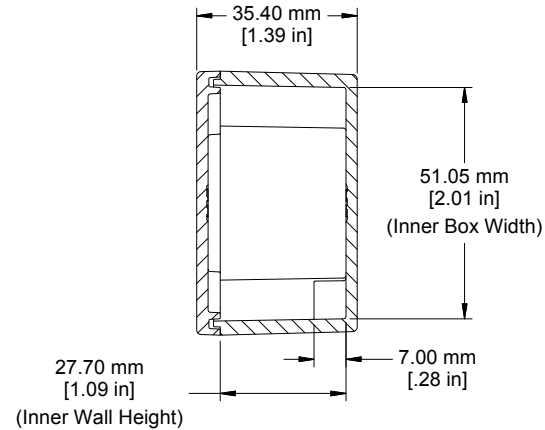
Top View Looking Inside Box
