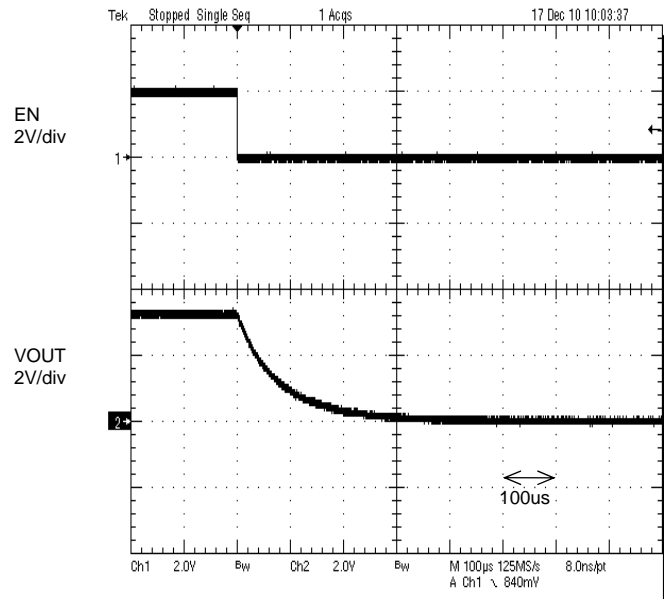
Figure 6. Shut down
