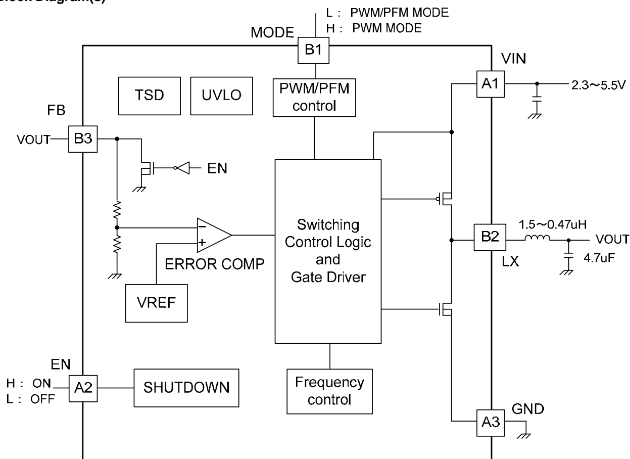
Figure 3. Block Diagram(s)
