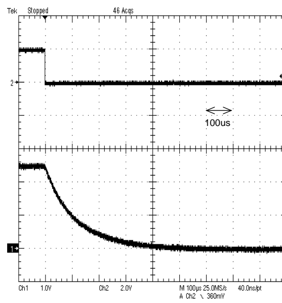
Figure 40. Shut down
