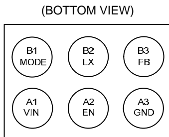
Figure 2. Pin Configuration(s)
