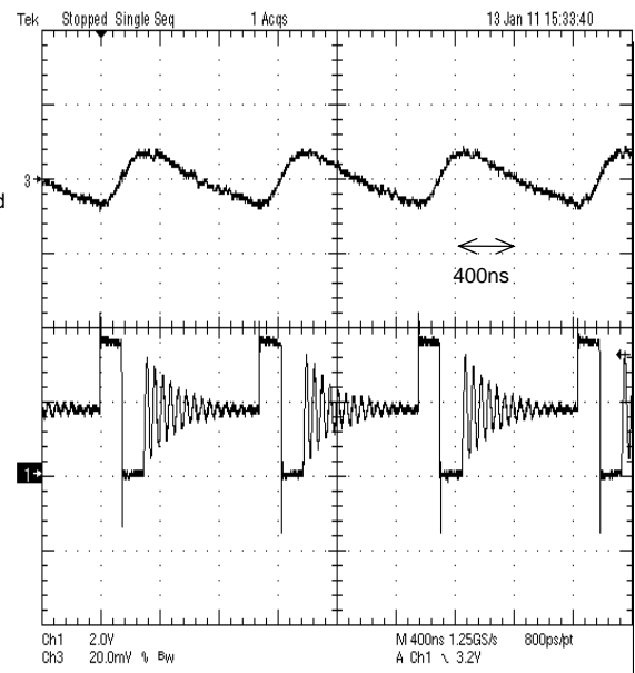
Figure 33. PFM mode Operation I_{out} = 50\text{mA}
