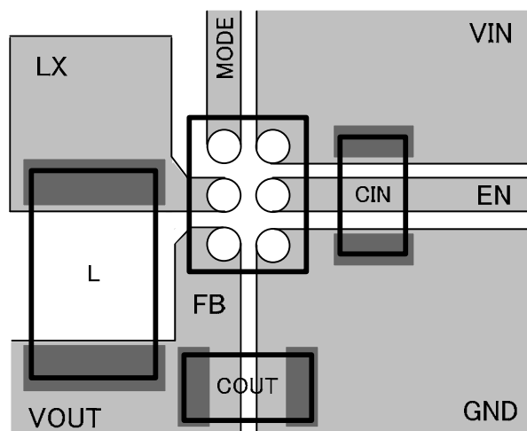
Figure 50. PCB layout
