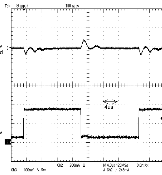
Figure 42. Load transient response 50mA to 350mA t_r=t_f=100\text{ns} , MODE : High
