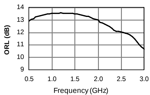
FIGURE 2. OUTPUT RETURN LOSS vs FREQUENCY
