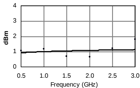
FIGURE 8. P1dB vs FREQUENCY
