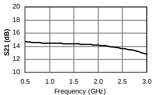
FIGURE 3. |S21| vs FREQUENCY
