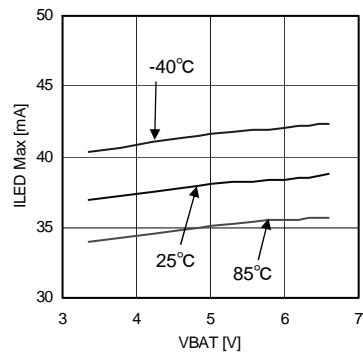
Fig 13. LED Max Current
