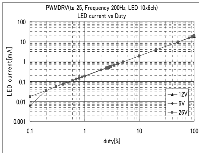
Fig.33 PWM characteristics of current driver PWM
