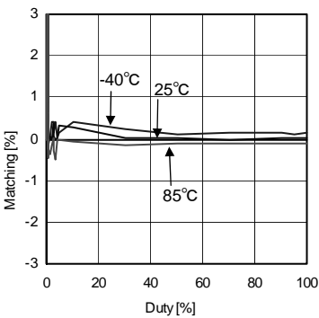
Fig 15. LED Current Matching
