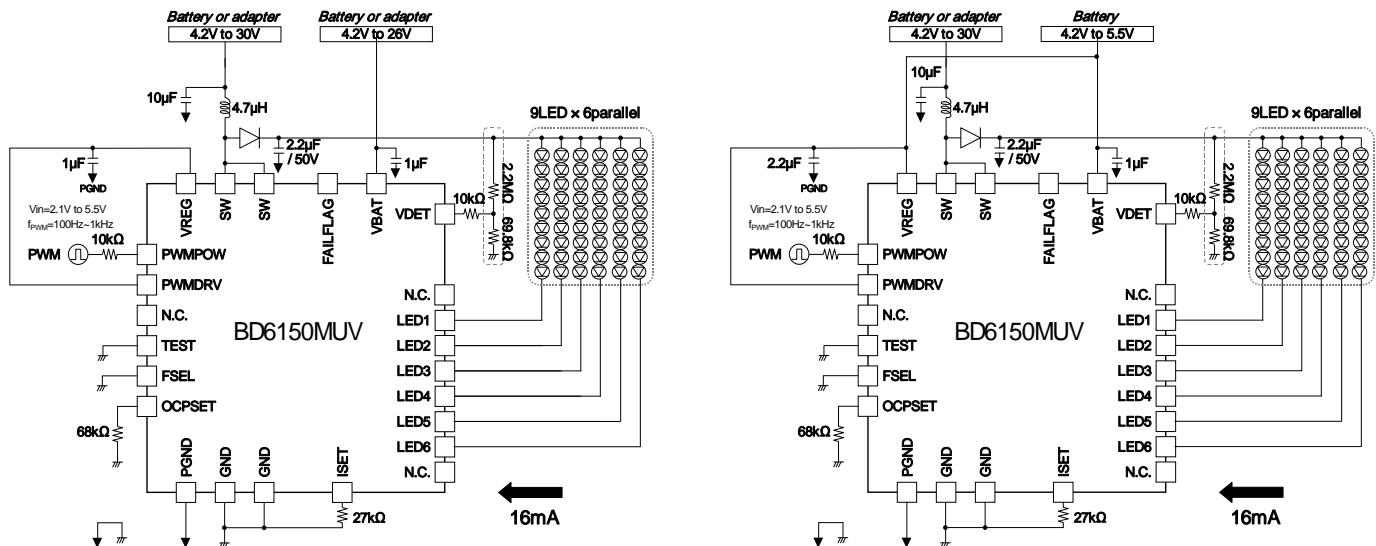
Fig.37 Application at the time of power supply isolation (6parallel)
