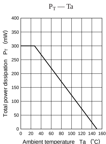
Characteristics charts of UN4211
