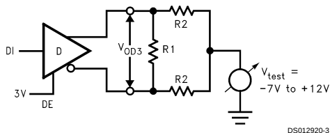
FIGURE 2. V_{OD3}
