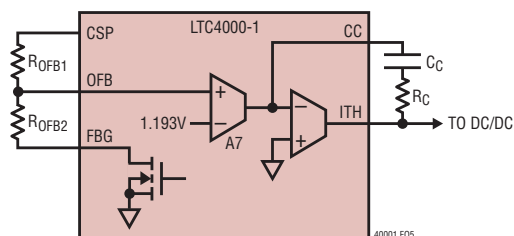
Figure 5. Output Voltage Regulation Loop with FBG
