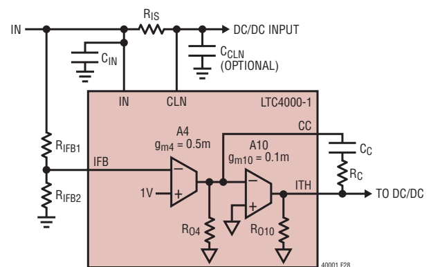
Figure 28. Simplified Linear Model of the Input Voltage Regulation Loop
