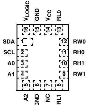
ISL23328 (16 LD UTQFN) TOP VIEW
