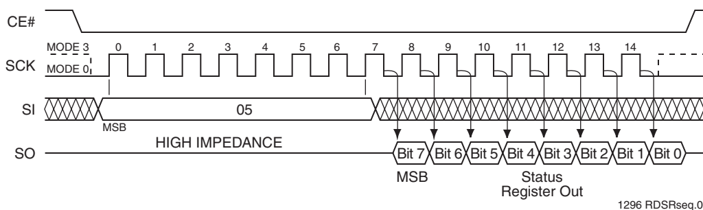
FIGURE 16: Read-Status-Register (RDSR) Sequence
