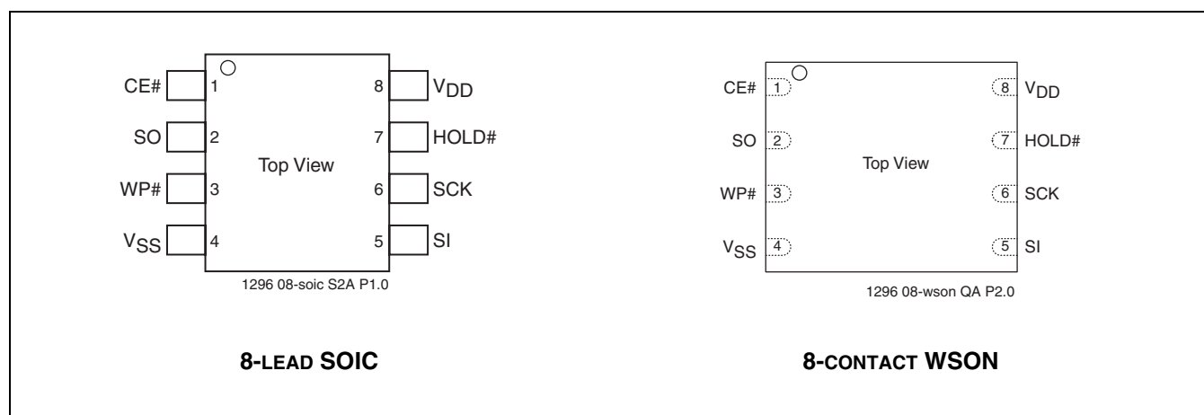
FIGURE 2: Pin Assignments
