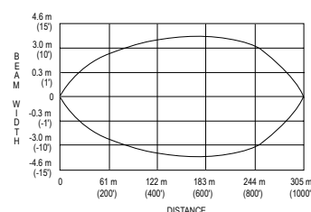
Figure 1. Beam Pattern
