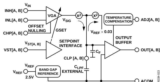
Figure 51. Single-Channel Details
