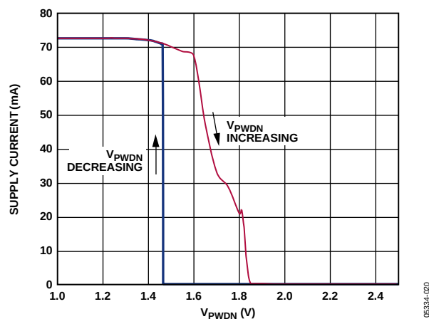
Figure 49. Supply Current vs. V_{PWDN}
