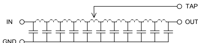
Functional Diagram
